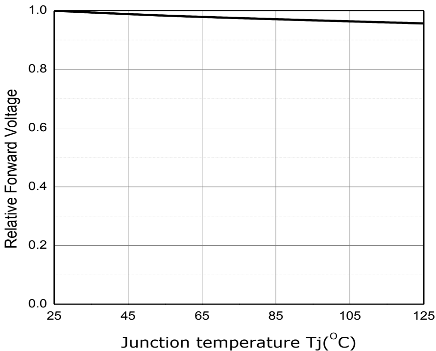
Fig 7. Junction Temperature vs. Relative Forward Voltage, I_F=60\text{mA}
