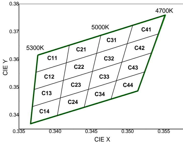
CIE Chromaticity Diagram (Cool white), T_j=25^\circ\text{C} , I_F=60\text{mA}
