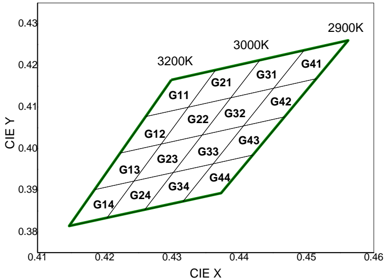
CIE Chromaticity Diagram (Warm white), T_j=25^\circ\text{C} , I_f=60\text{mA}
