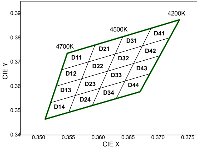
CIE Chromaticity Diagram (Neutral white), T_j=25^\circ\text{C} , I_f=60\text{mA}
