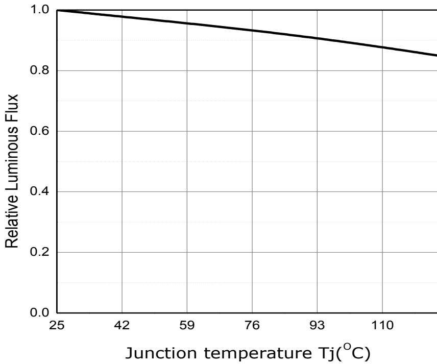
Fig 6. Junction Temperature vs. Relative Luminous Flux, I_F=60\text{mA}
