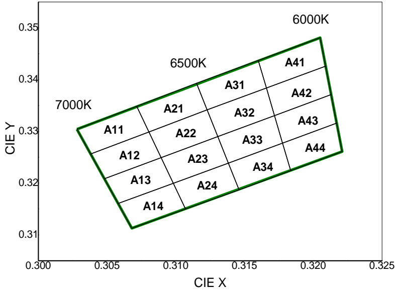
CIE Chromaticity Diagram (Cool white), T_j=25^\circ\text{C} , I_F=60\text{mA}
